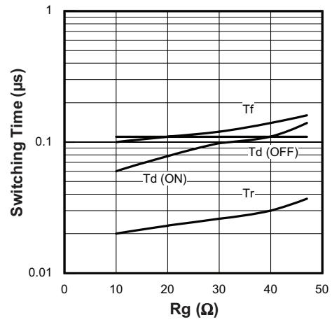
Fig. 8 - Typical Switching Time vs. R_G T_J = 125\text{ }^\circ\text{C} ; L = 200\text{ }\mu\text{H} ; V_{CE} = 600\text{ V} I_{CE} = 20\text{ A} ; V_{GE} = 15\text{ V}
